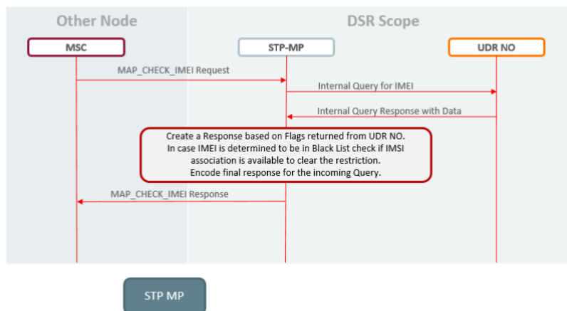
Figure 79 – SS7 EIR call flow
