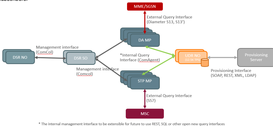
Figure 78 – EIR solution architecture.
