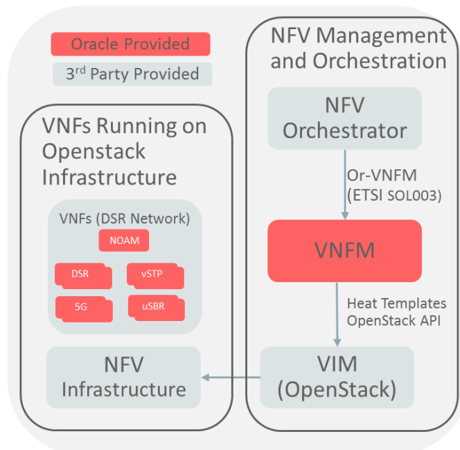
Figure 71 – DSR VNFM
