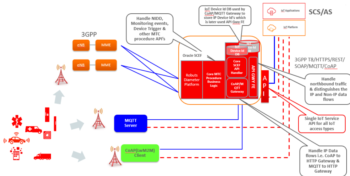
Figure 69: SCEF LWM2M Server, MQTT architecture example
