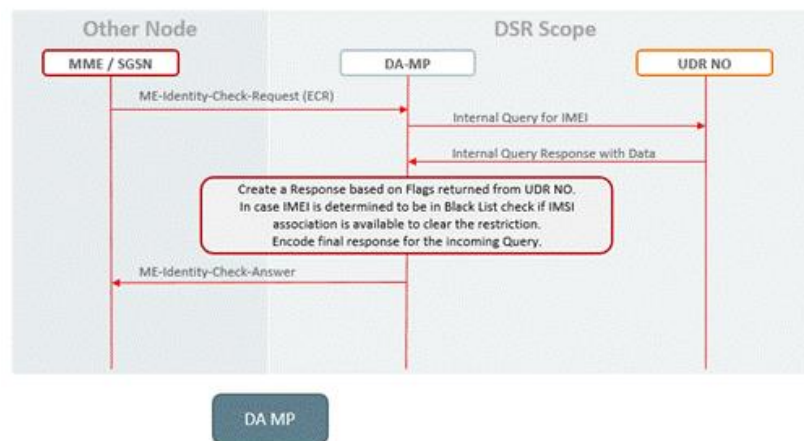
Figure 80 – S13 EIR Call Flow
